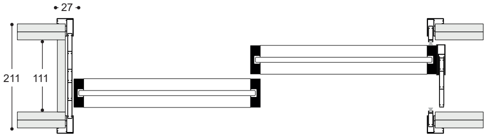
JAMBA CASONETO PARA 2 PANELES CORREDEROS, CON TAPAEMBOCADURA. JAMB FOR 2 SLIDING PANELS, WITH COVER.
