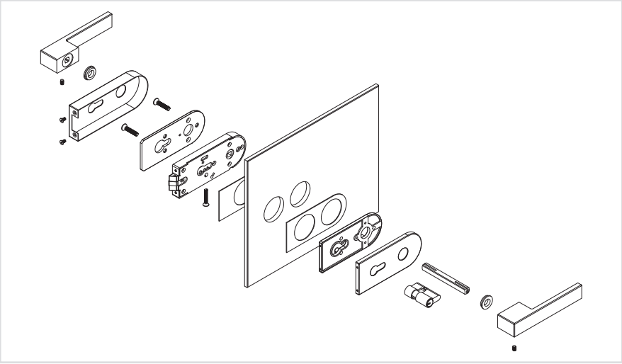
Usar tornillo suministrado M5x35mm Use supplied screw M5x35mm
