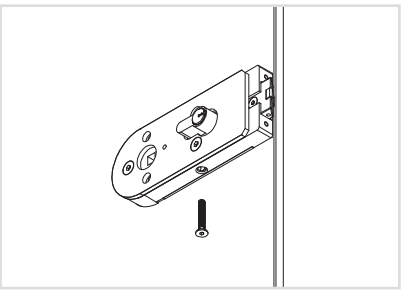
Usar tornillo suministrado M5x35mm Use supplied screw M5x35mm
